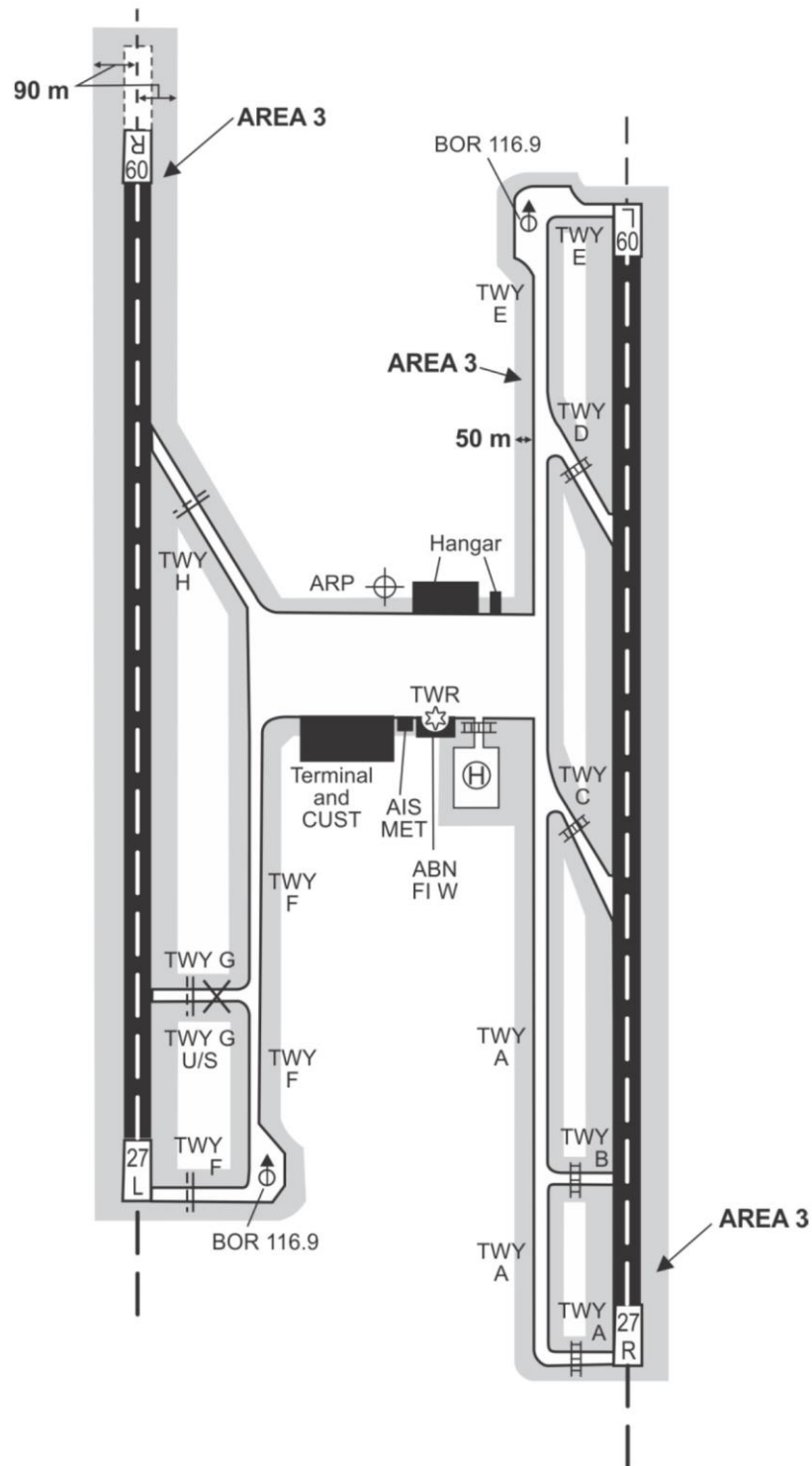
Terrain and obstacle data collection surface — Area 3
